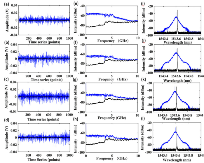
Fig. 3. Chaotic time series (a) (b) (c) (d), corresponding RF spectra (e) (f) (g) (h) and optical spectra (i) (j) (k) (l). Black lines in each figures represent the situation without feedback. (a) (e) (i) represents chaotic system without FDGD. (b) (f) (j) represent chaotic system with FDGD where the group delay curve is linear within the chaotic spectrum with a 2000ps/nm dispersion. (c) (g) (k) represents chaotic system with FDGD where the group delay curve is linear within the chaotic spectrum with a 1000ps/nm dispersion. (d) (h) (l) represents chaotic system with FDGD where the group delay curve is irregular within the chaotic spectrum.
